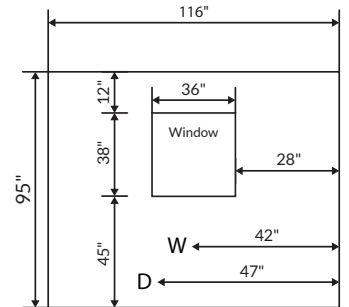
Example 2, Elevation
